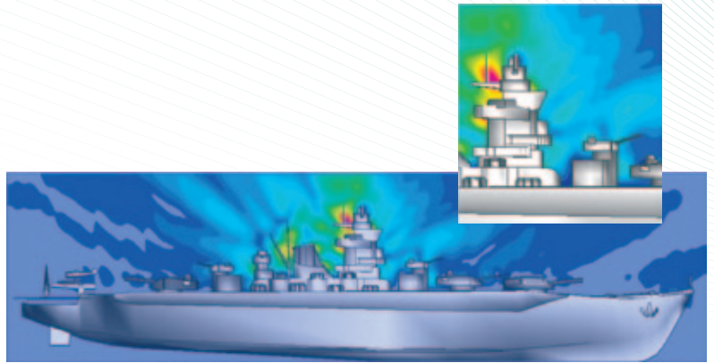
Antenna radiation
